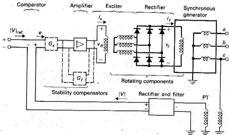
Figure 9-2 Brushless AVR loop.
